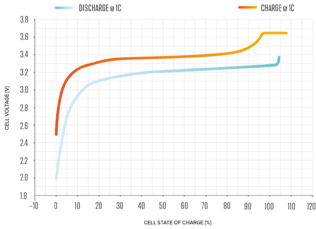
TYPICAL CHARGE & DISCHARGE VOLTAGE VS CHARGE STATE (SoC) CURVE OF A LiFePO 4 CELL (25 °C)
